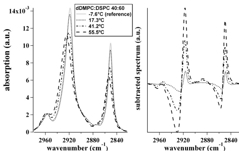
Fig. 2. The IR absorption spectrum contains different absorption maxima originating from varying vibrations. In the left panel the asymmetric and the symmetric CH_2 stretch vibrations as measured in a sample of DMPC-d54:DSPC 40:60 at different temperatures are displayed. The absorption maxima of these are temperature dependent and lie at around 2852\text{ cm}^{-1} (symmetric) and at 2925\text{ cm}^{-1} (asymmetric). The asymmetric and symmetric CD_2 stretch vibrations are shifted to lower wavenumbers due to the heavier deuterium atoms ( data not shown ). In previous studies from other labs the melting processes were investigated following the temperature dependence of the absorption maxima. In this study, however, the melting process was also studied by defining a reference spectra (here taken at a temperature of -7.6 °C) and subtracting this one from all other spectra where in each case the area was normalized to 1\text{ cm}^{-1} ( Difference Spectra method ). Example results of the difference spectra of the left panel are displayed in the right panel. As a measure of the progress of the melting process the area of one of the peaks was taken.
